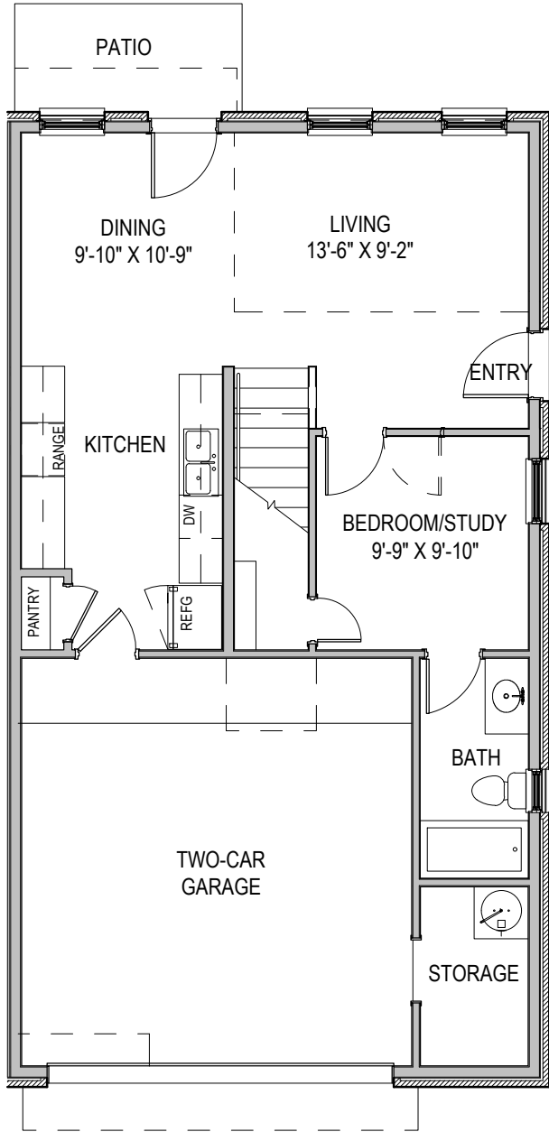
FIRST FLOOR
